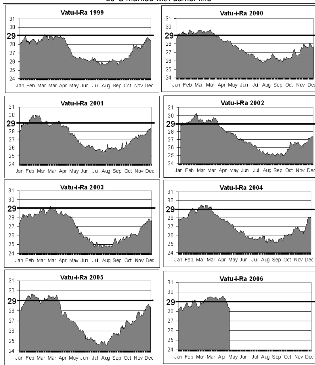
Figure 4.1: Graphs of water temperatures, Vatu-i-Ra Passage 1999 – mid 2006
